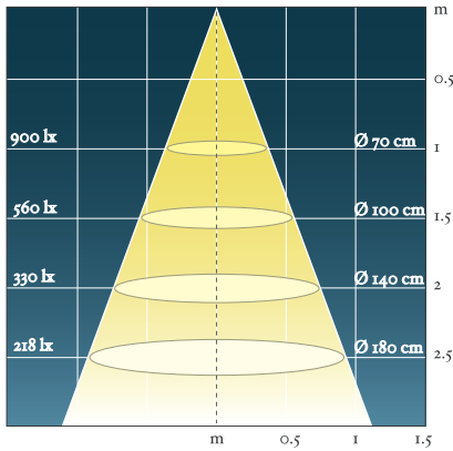
LED reflector, HALOLED- E27, 12W -warm white, 40°
